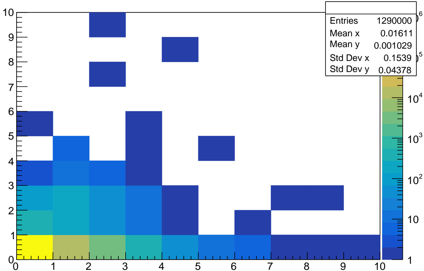
ClusterSize[0][0]:ClusterNumber[0][0] {Ev_Num<10000}
