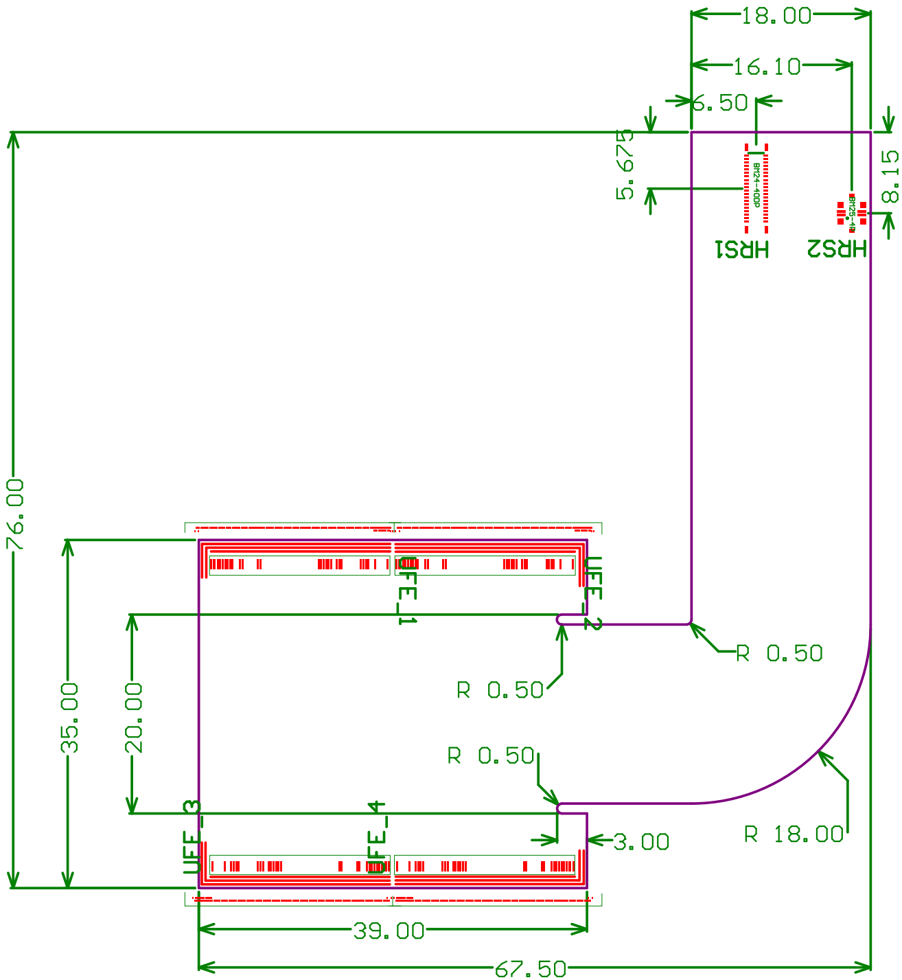
KEK Quad Type-C
